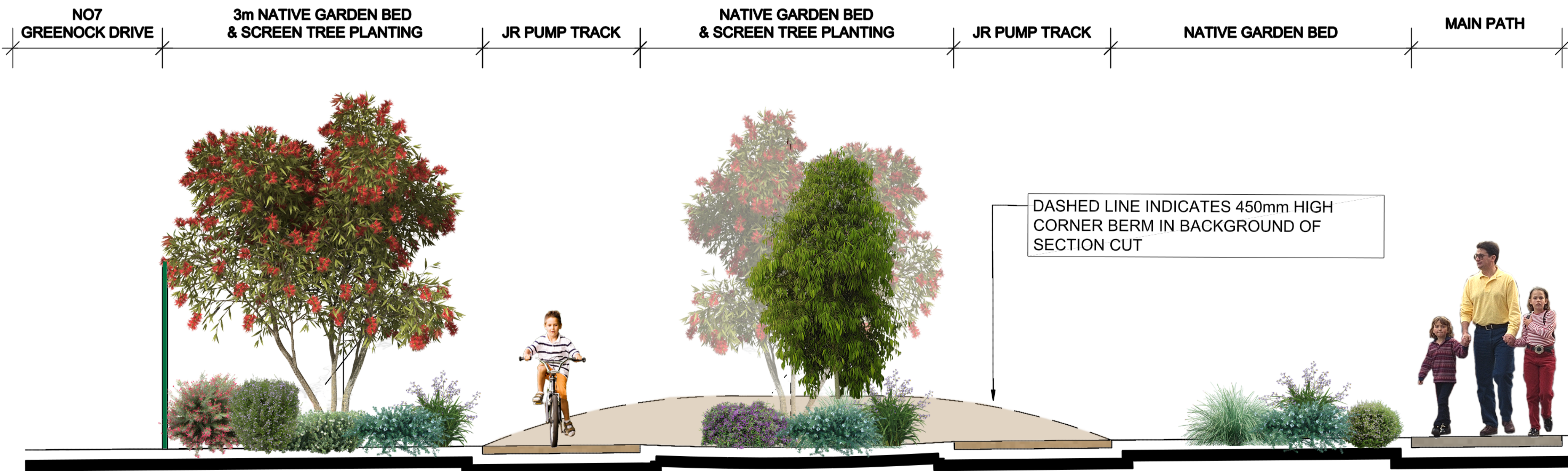
SECTION B-B
