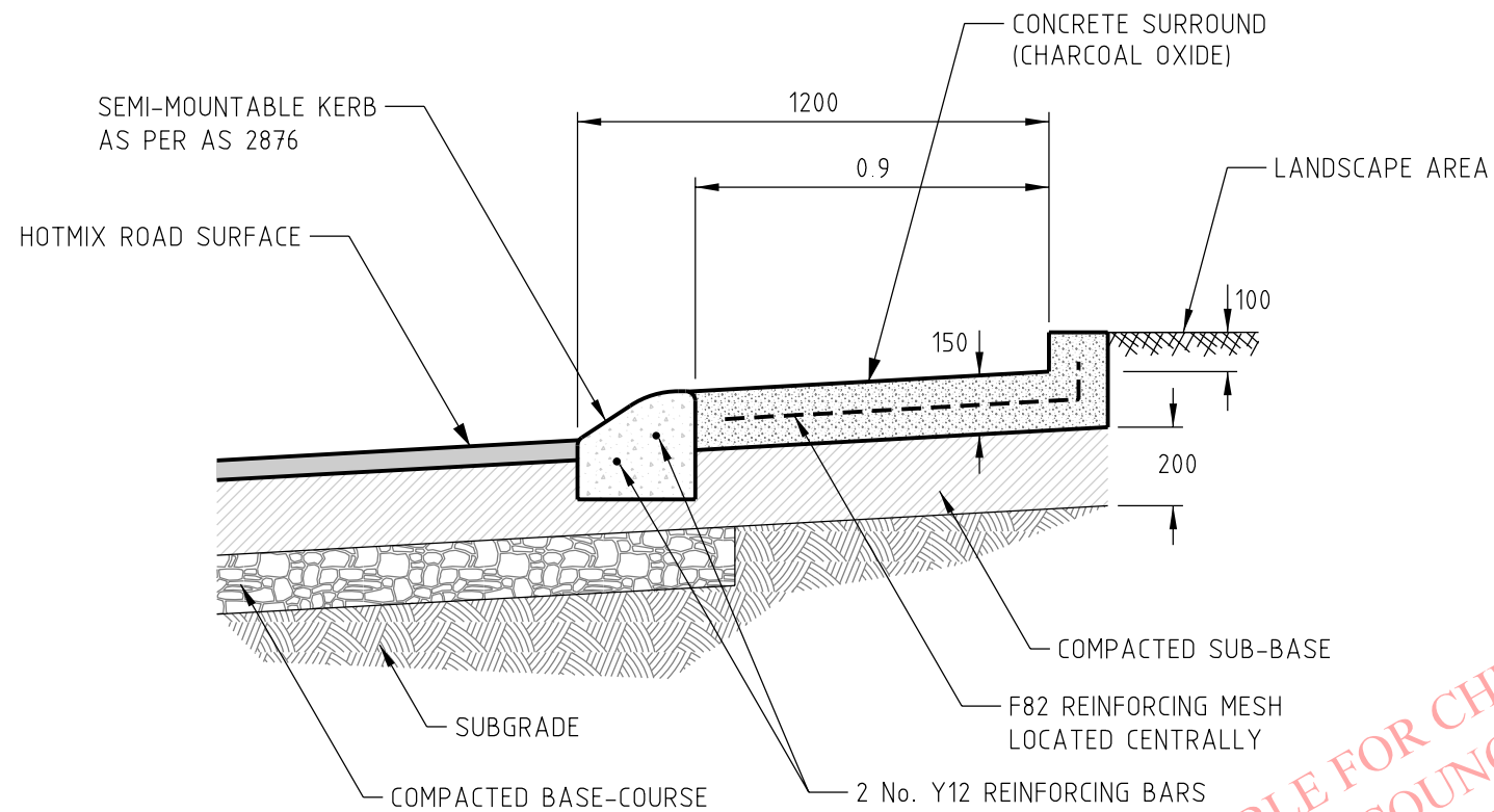
TYPICAL ROUNDABOUT SURROUND CROSS-SECTION
