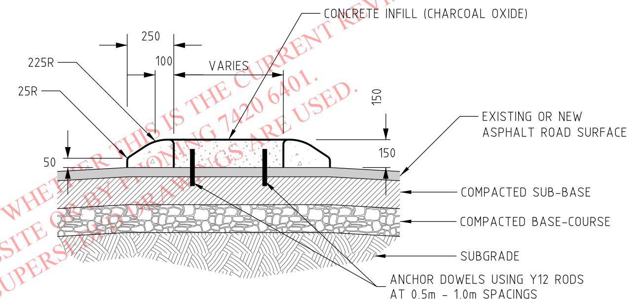
TYPICAL SPLITTER ISLAND & TRAFFIC ISLAND DETAIL CAST ON TOP OF FINISHED ROAD SURFACE
