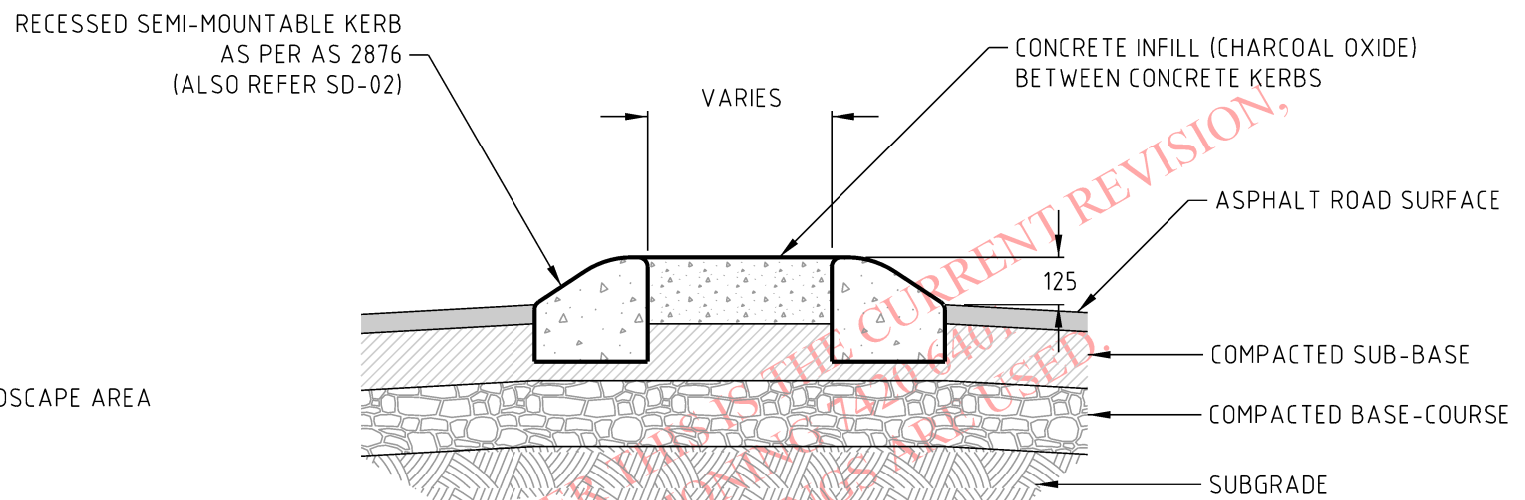
TYPICAL (PREFERRED) SPLITTER ISLAND & TRAFFIC ISLAND DETAIL WITH RECESSED SEMI-MOUNTABLE KERB
